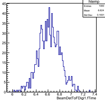
BeamDetToFdigi1.fTime
