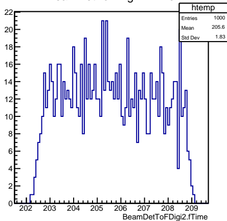
BeamDetToFdigi2.fTime
