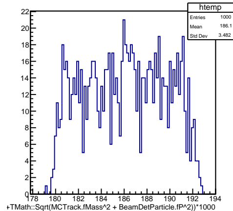
((MCTrack.fMass+TMath.Sqrt(MCTrack.fMass^2 + BeamDetParticle.fP^2))*1000 (MCTrack.fPdgCode == 1000020960)
