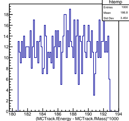
(MCTrack.fEnergy - MCTrack.fMass)*1000 (MCTrack.fPdgCode == 1000020960)
